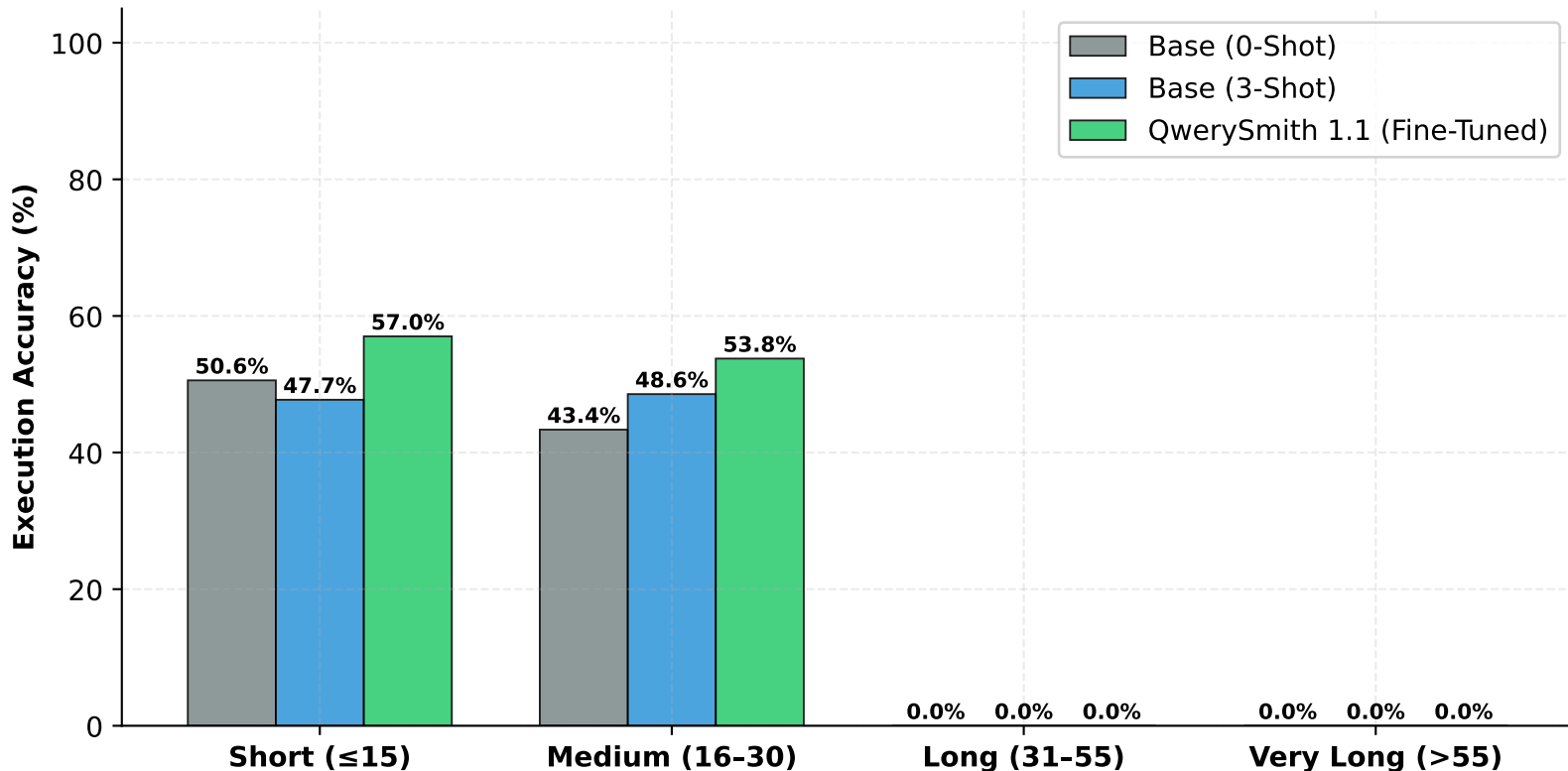
Figure 13: SQL Token Length vs. Execution Accuracy Stratification
