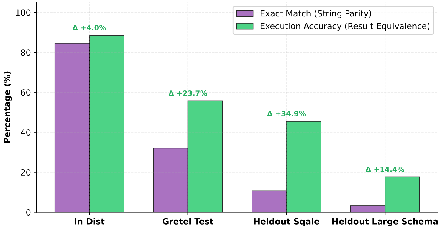
Figure 2: Exact Match vs. Execution Accuracy (Semantic Generalization Gap)
