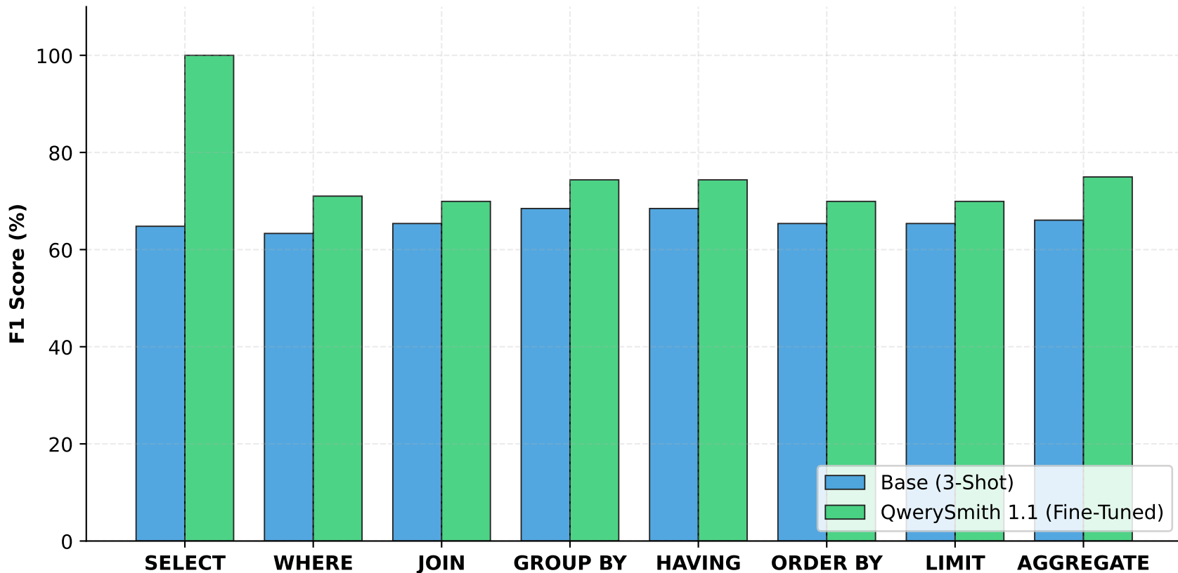
Figure 3: AST Clause Detection F1 Score Across Key SQL Constructs
