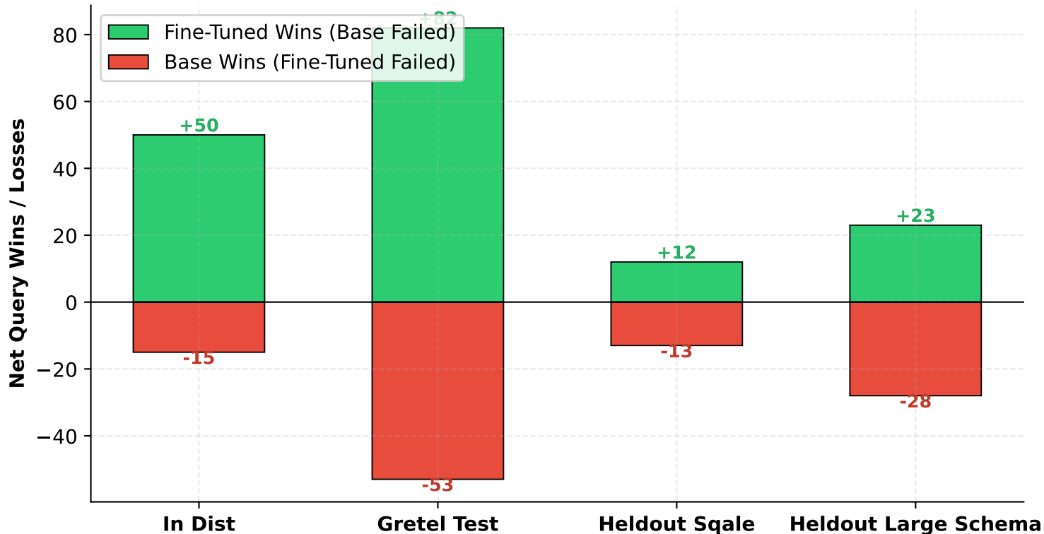
Figure 4: Pairwise Head-to-Head Win/Loss Margin (Fine-Tuned vs 3-Shot Base)
