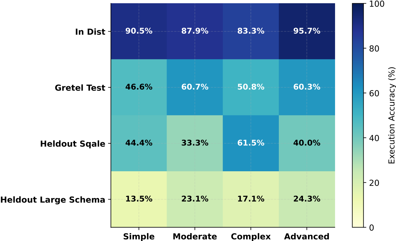
Figure 9: Execution Accuracy Stratification by SQL Complexity Tier
