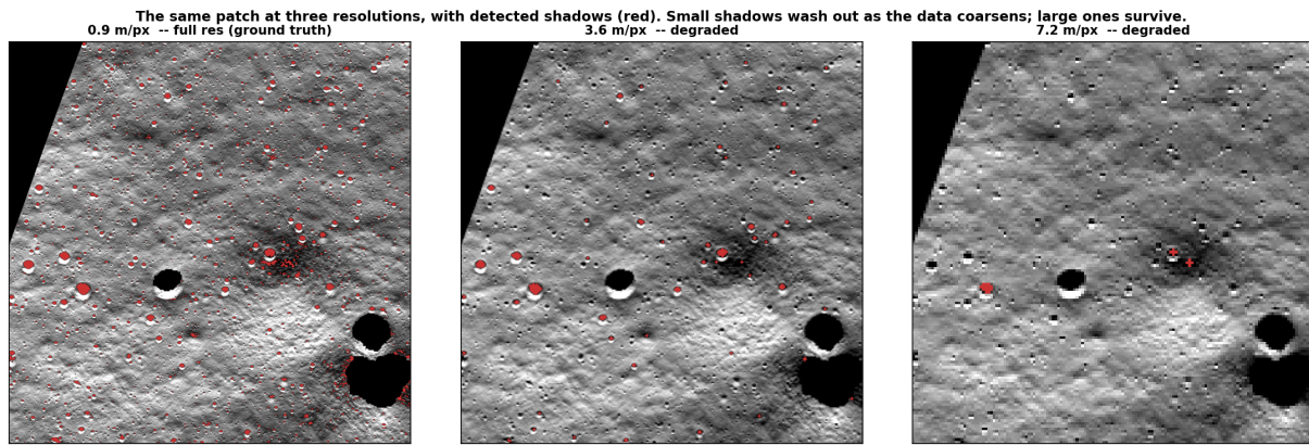
Figure 14: The same patch at 0.9, 3.6, and 7.2 m/px, with detected shadows in red. Small shadows wash out as the data coarsens; large ones survive — the reach curve made visible.
