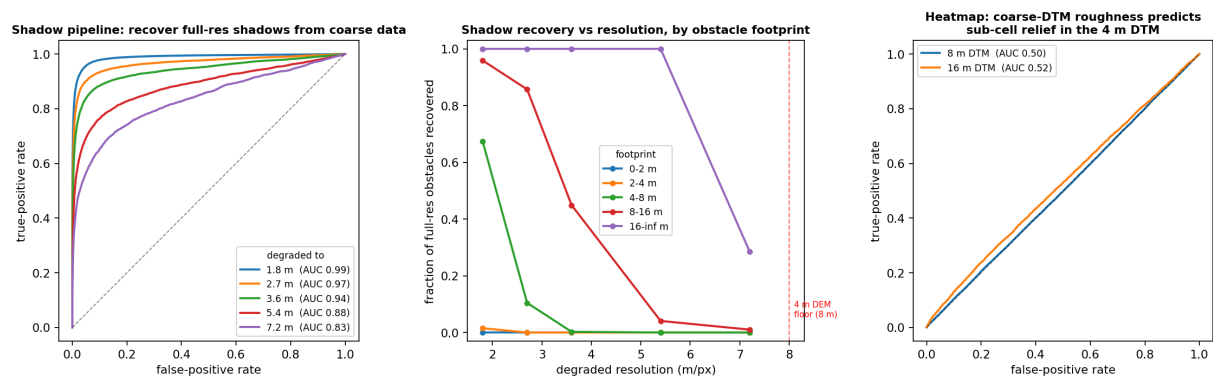
Figure 12: Shadow-channel validation. Left: detection ROC at each degraded resolution. Centre: the reach curve — fraction of full-resolution obstacles recovered versus resolution, by footprint. Right: the first, naive heatmap test, sitting on the chance diagonal (an information boundary, not a fault).
