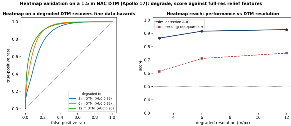
Figure 13: Heatmap validation done properly, on a 1.5 m NAC DTM (Apollo 17): degrade the model, score the coarse heatmap against the relief features the fine model resolves. Detection AUC 0.86–0.93 across 3–12 m.
