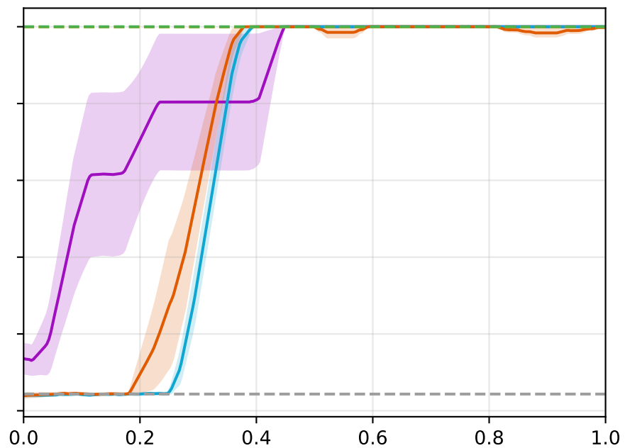
Acrobot-v1 — K = 15
