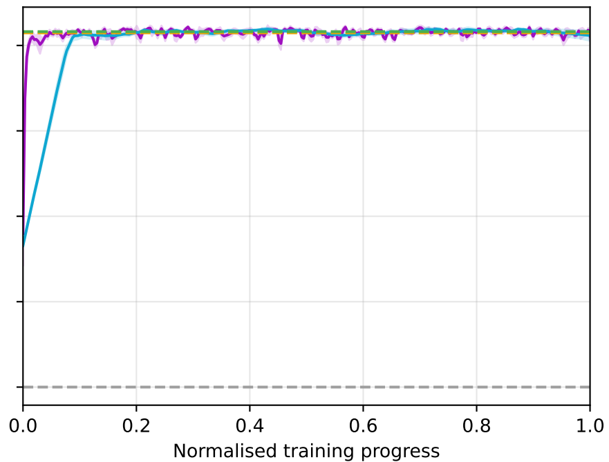
Acrobot-v1 — K = 15
