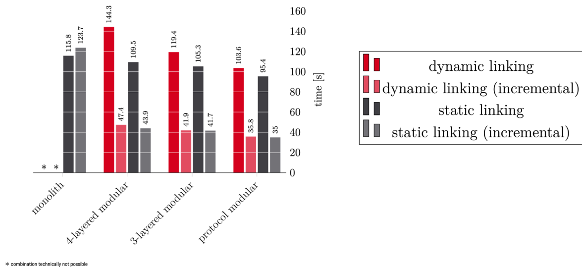
Figure 16 – Compile time benchmarking results
