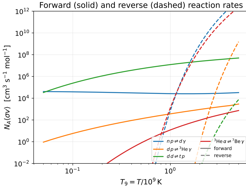
Figure 7: Forward (solid) and reverse (dashed, by detailed balance) rates N_A\langle\sigma v\rangle(T_9) for four key reactions. The forward rates depend only weakly on T_9 ; the reverse photo-dissociation rates rise steeply and cross the forward rates near T_9 \sim 1 –2.
