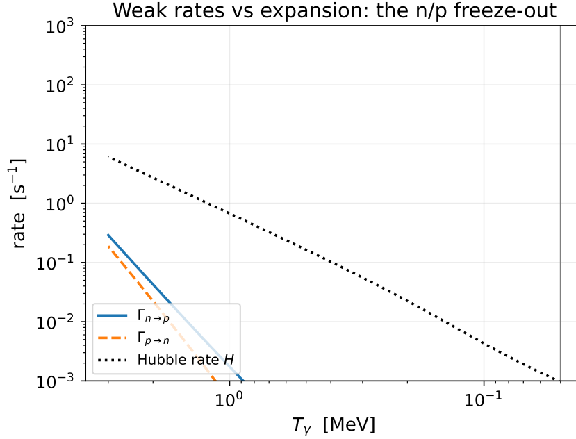
Figure 4: Calibrated weak rates and the Hubble rate H . Equilibrium holds where \Gamma > H ; the high- T crossing is the n/p freeze-out. (Time flows left to right.)
