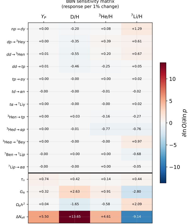
Figure 10: Logarithmic sensitivity \partial \ln O / \partial \ln p of the four observables (columns) to the nuclear rates (top block) and physical parameters (bottom block), per 1% change. Red is positive, blue negative.
