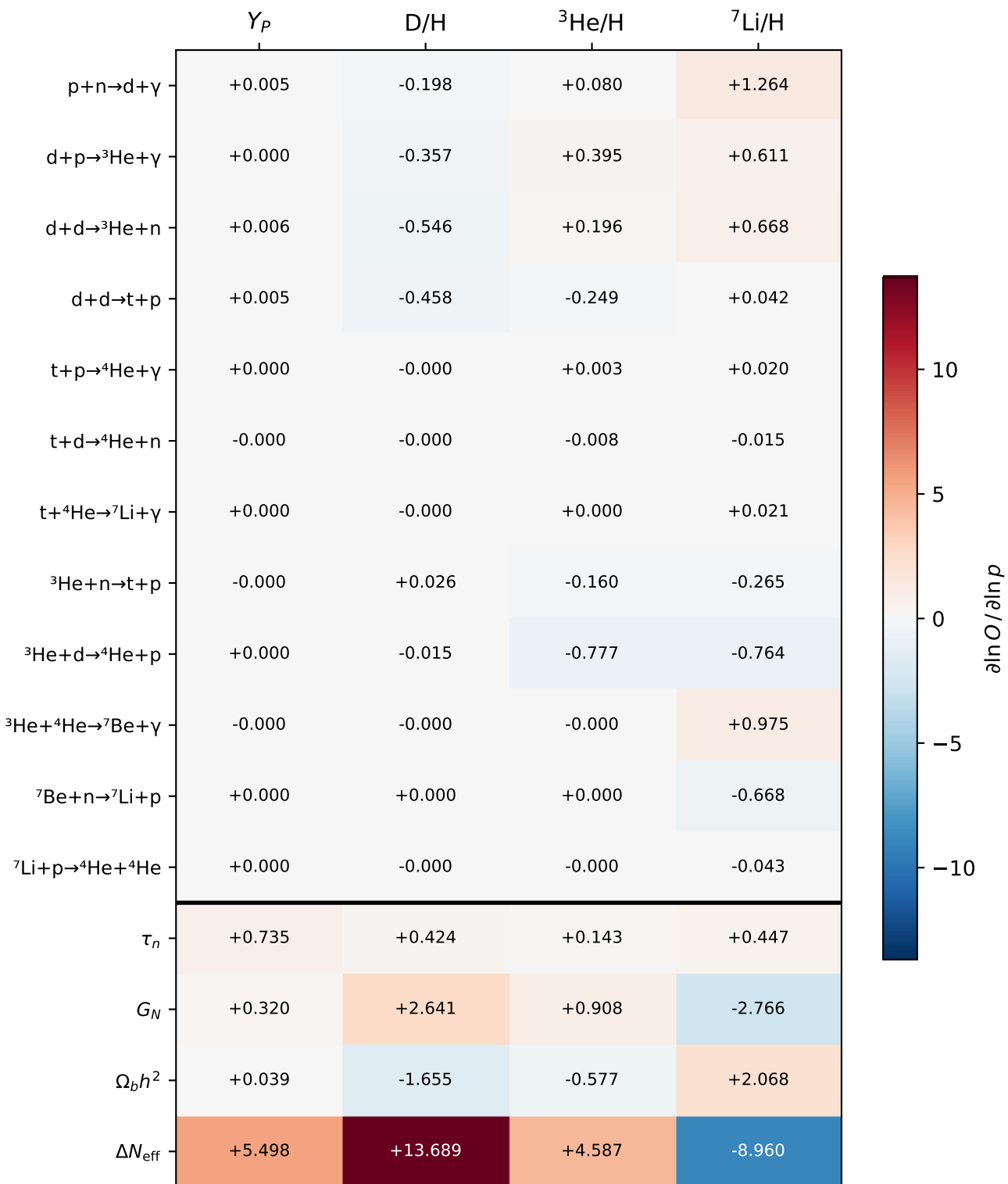
BBN sensitivity matrix (per 1% change)
