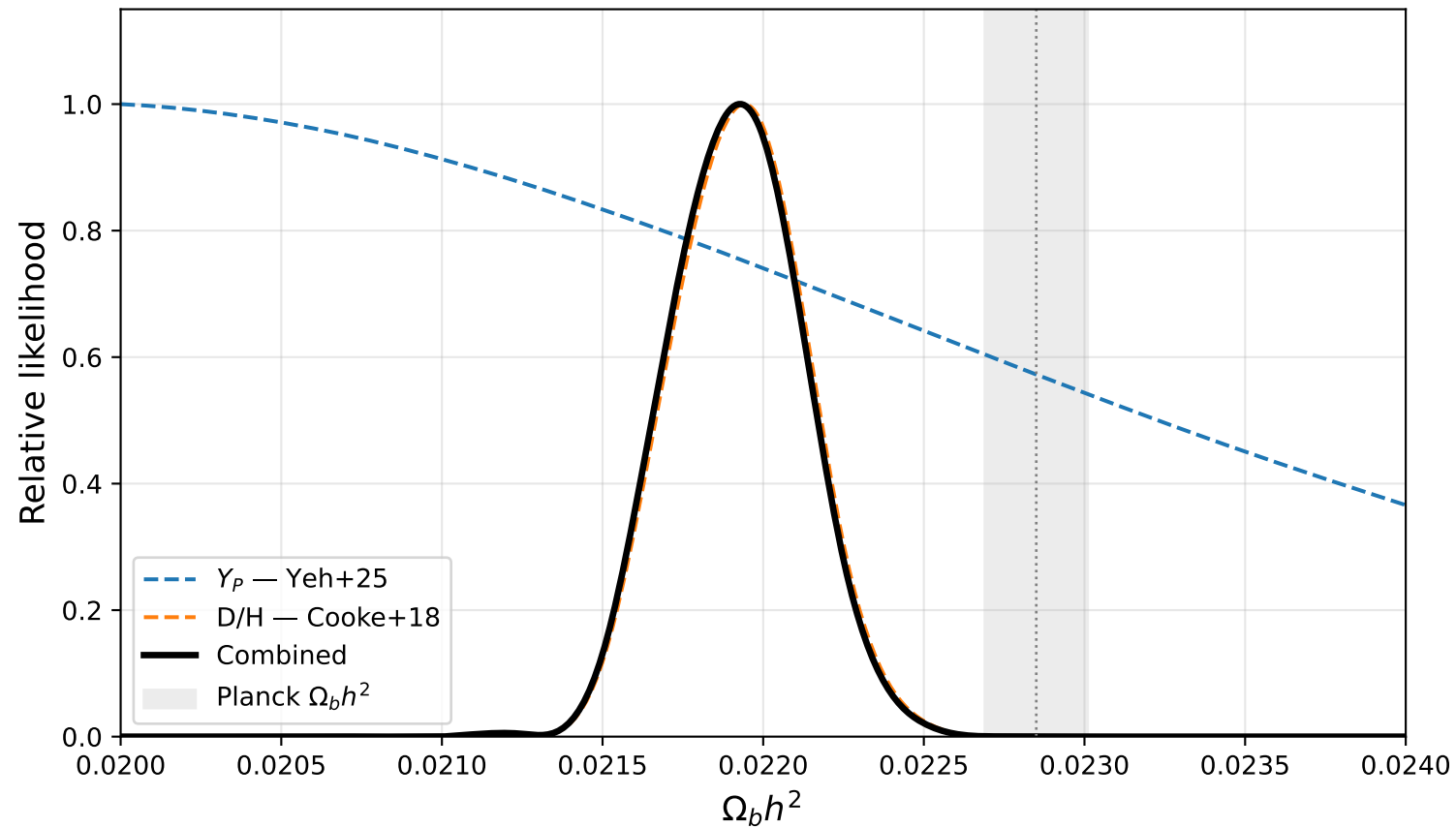
Posterior on \Omega_b h^2 from Y_p and D/H
