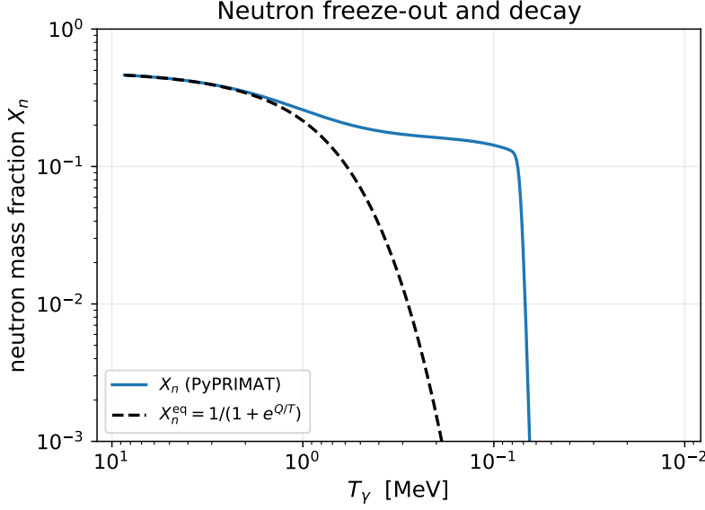
Figure 6: Neutron mass fraction X_n from PyPRIMAT (solid) versus the weak-equilibrium prediction X_n^{\text{eq}} = 1/(1 + e^{Q/T}) (dashed). X_n tracks equilibrium until freeze-out near 0.8 MeV, then declines slowly until deuterium formation burns the neutrons into {}^4\text{He} .
