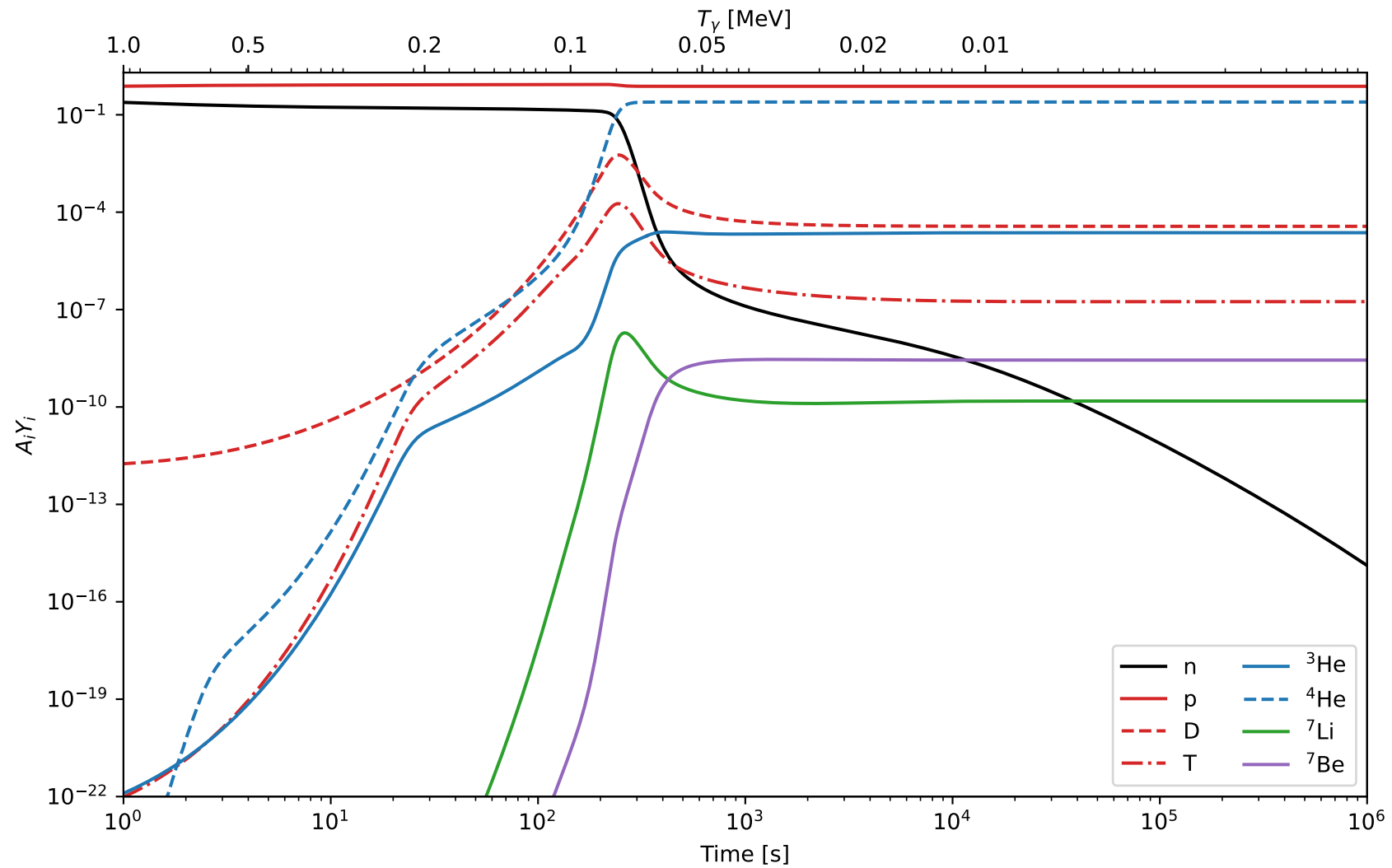
BBN abundance evolution — small network
