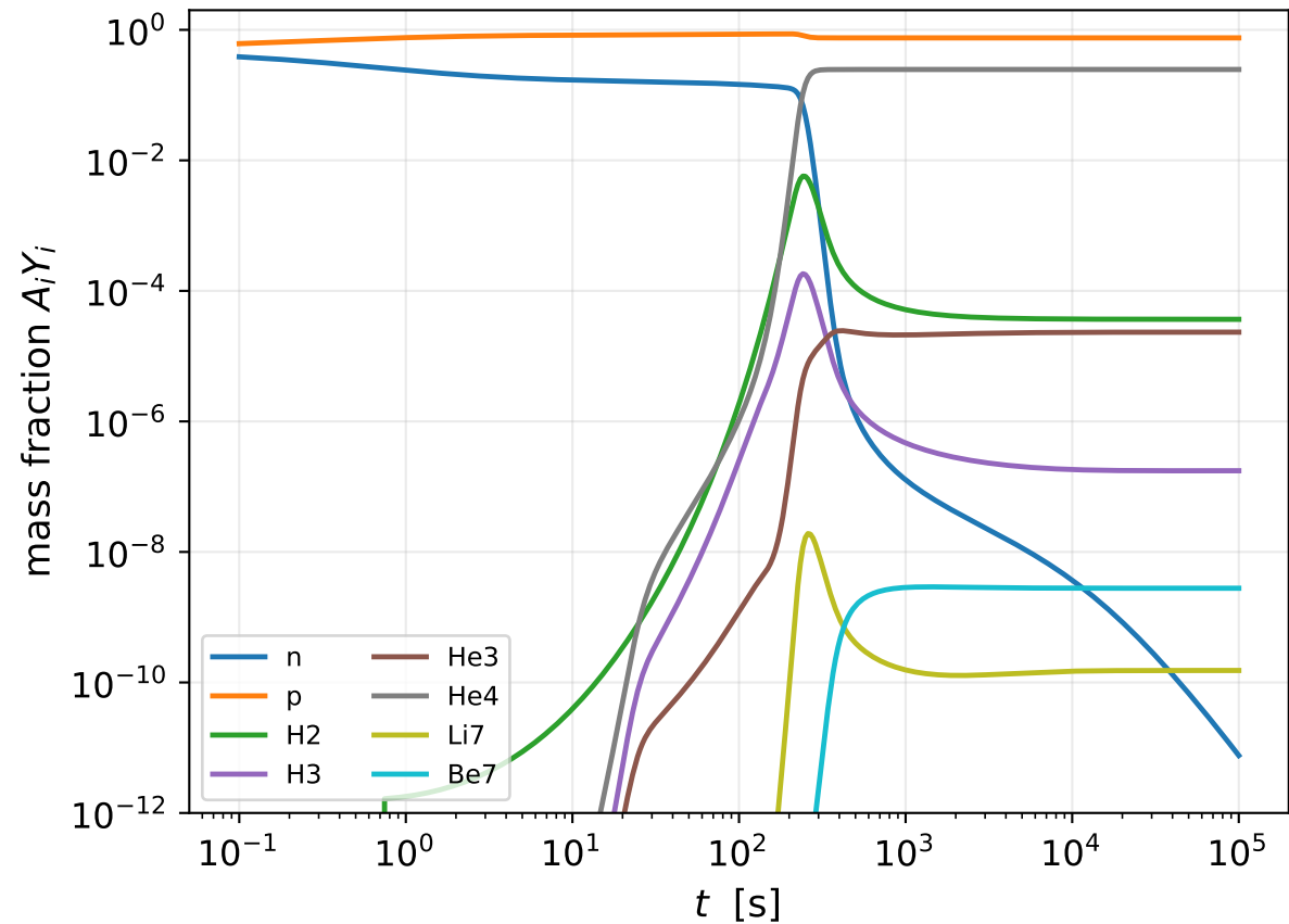
Abundance evolution (small network)
