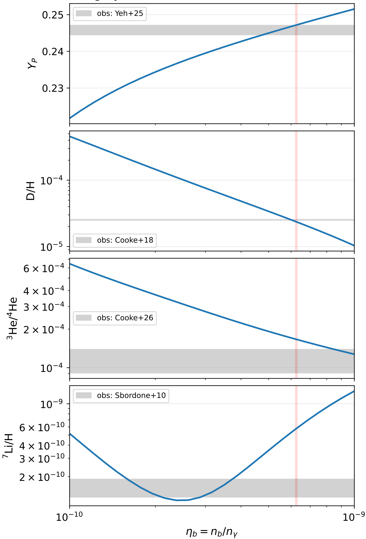
Schramm diagram with observational constraints (grey: measured value; red: Planck \Omega_b h^2 )
