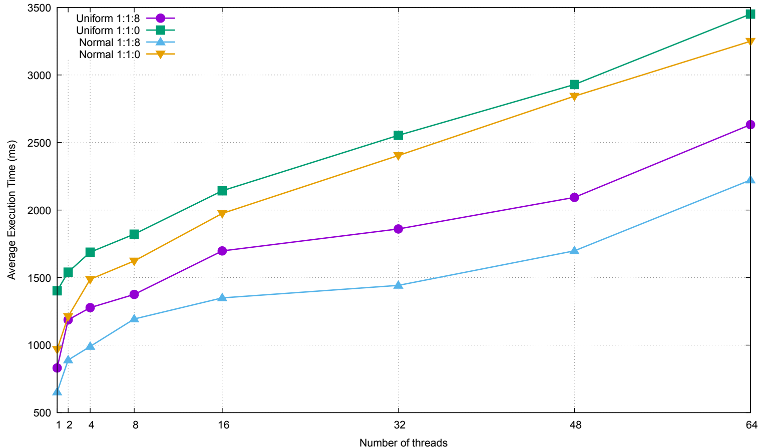
Execution Time vs Threads (LockFreeSkipList)
