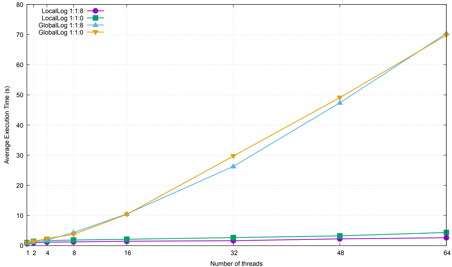
Execution Time vs Threads (Normal Distribution)
