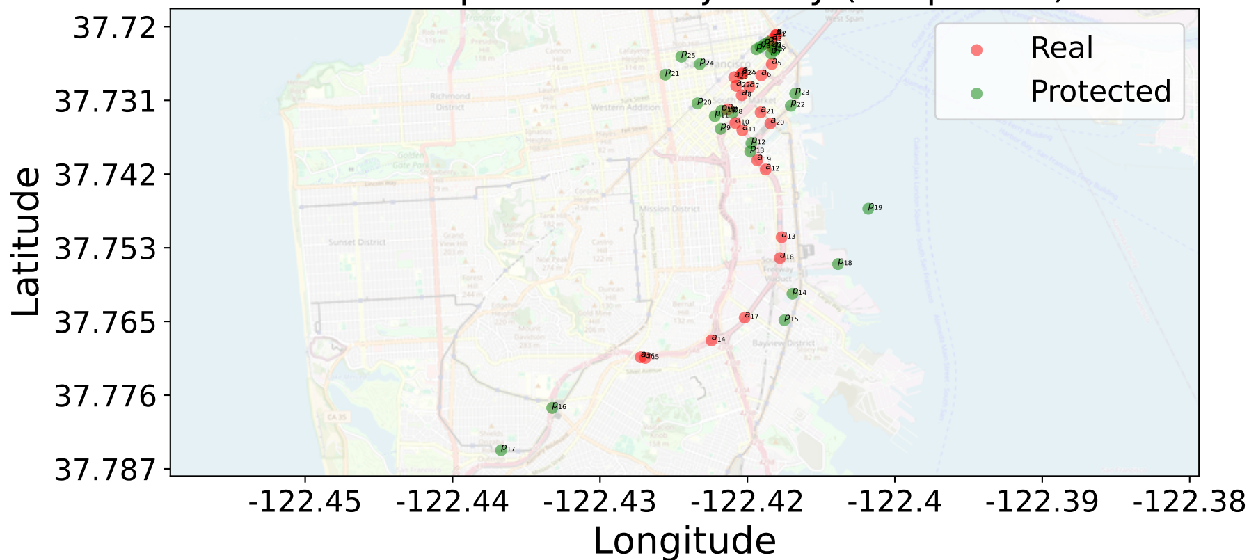
Real vs. protected trajectory (adaptive k)
