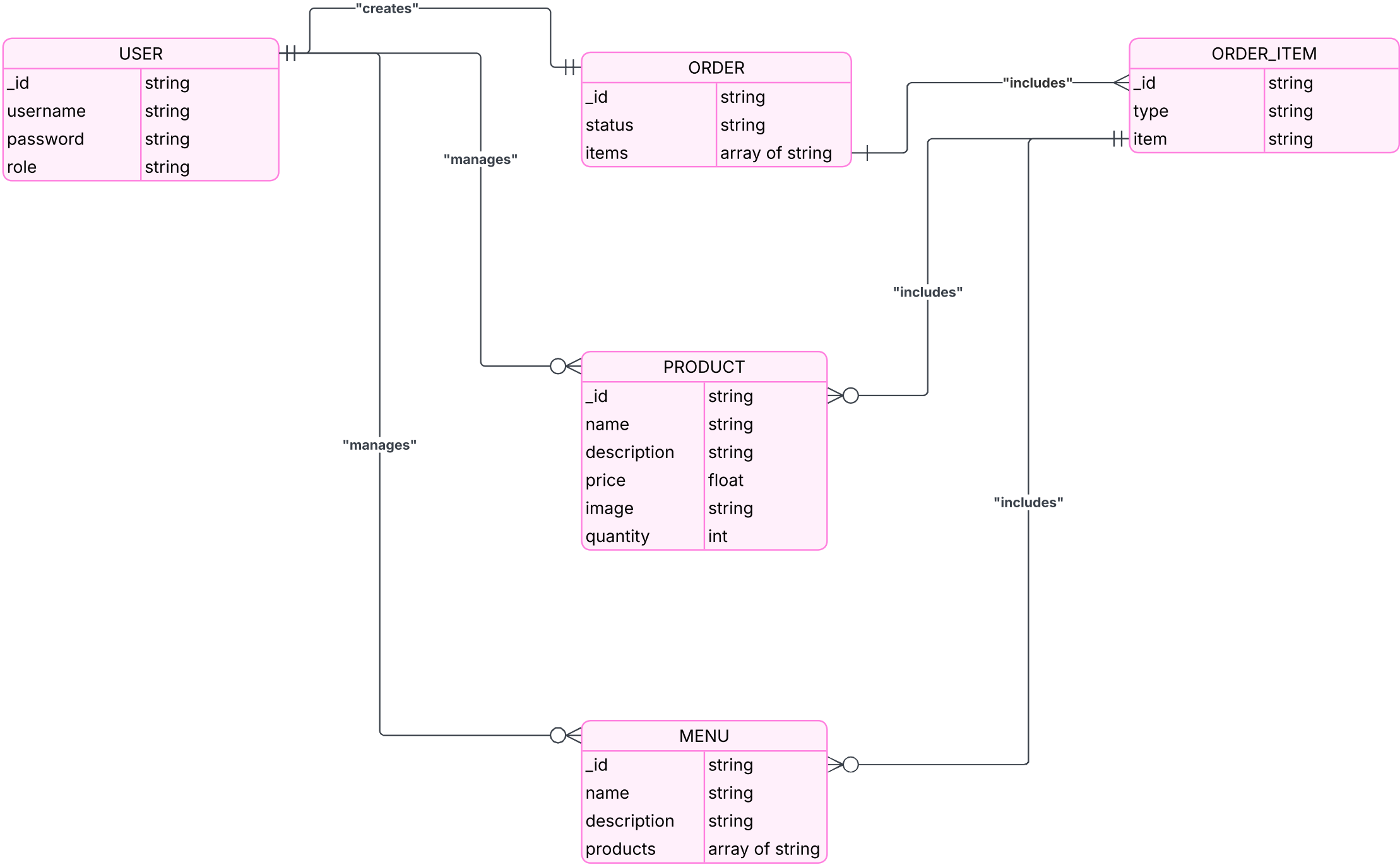
Retail/Restaurant Management ER Diagram
