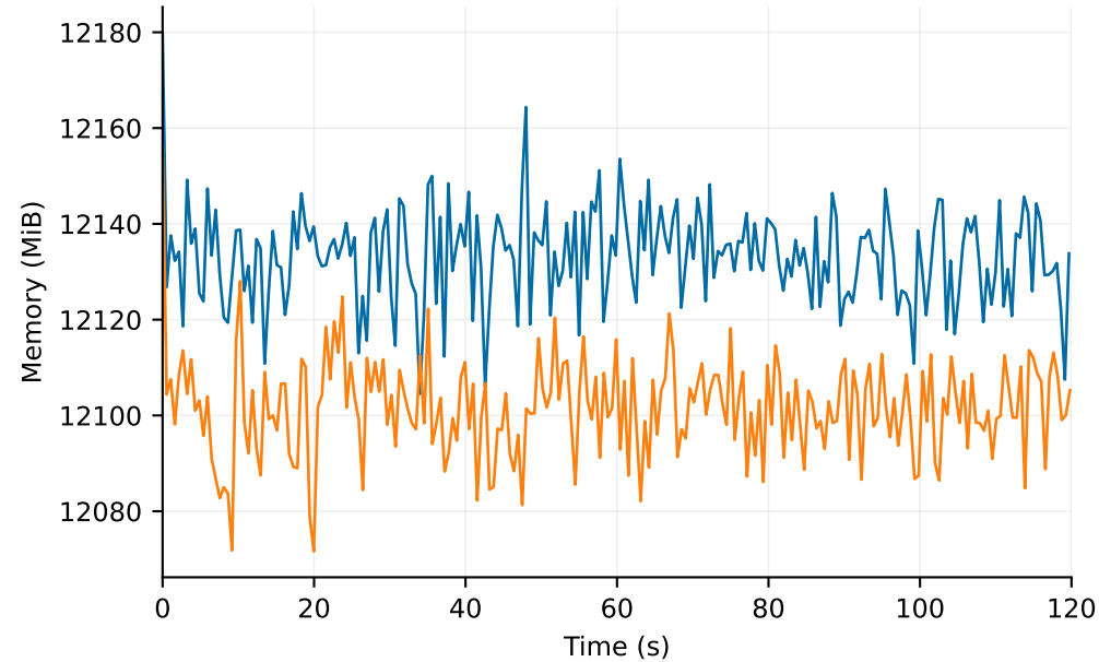
System MemAvailable
