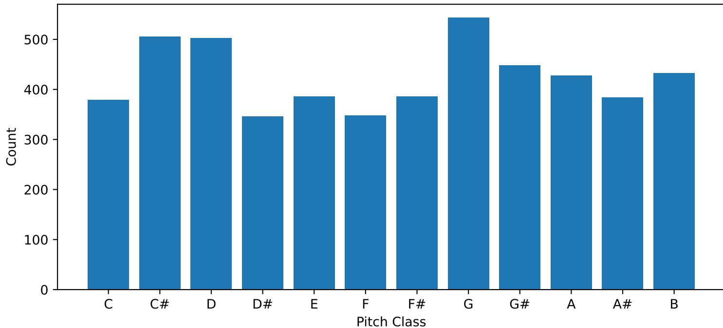
Pitch Class Distribution
