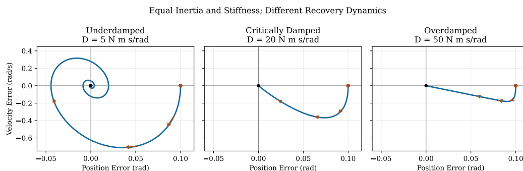
Figure 31.1: Manufactured Recovery With Equal Inertia and Stiffness: Only the Underdamped Case Spirals. All Curves Start at 0.1 rad With Zero Velocity; Orange Arrows Indicate Time Direction Over a Two-Second Interval.
