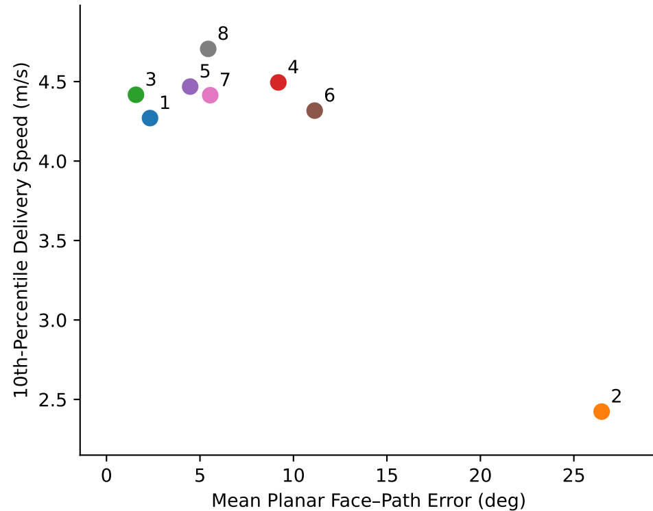
Speed Versus Planar Error
