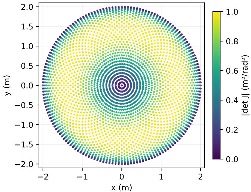
Position-Jacobian Area Scaling
