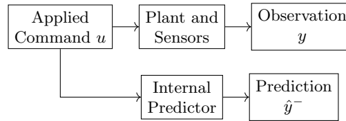
Figure 5.1: An Engineering Separation of Plant and Predictor. An Internal Command Copy Can Inform Prediction; the Physical Command Acts Through the Plant.
