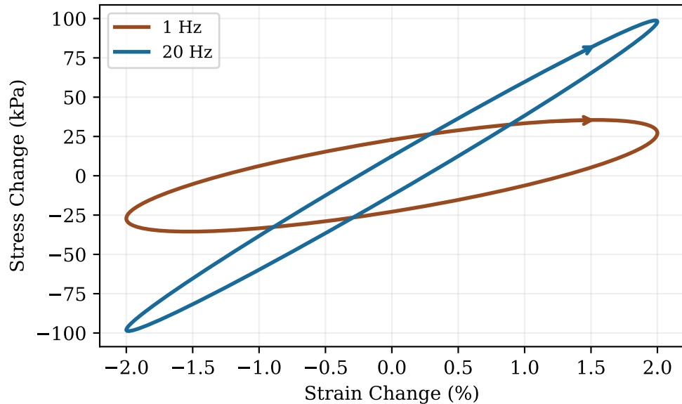
Cyclic Perturbation: Hysteresis
