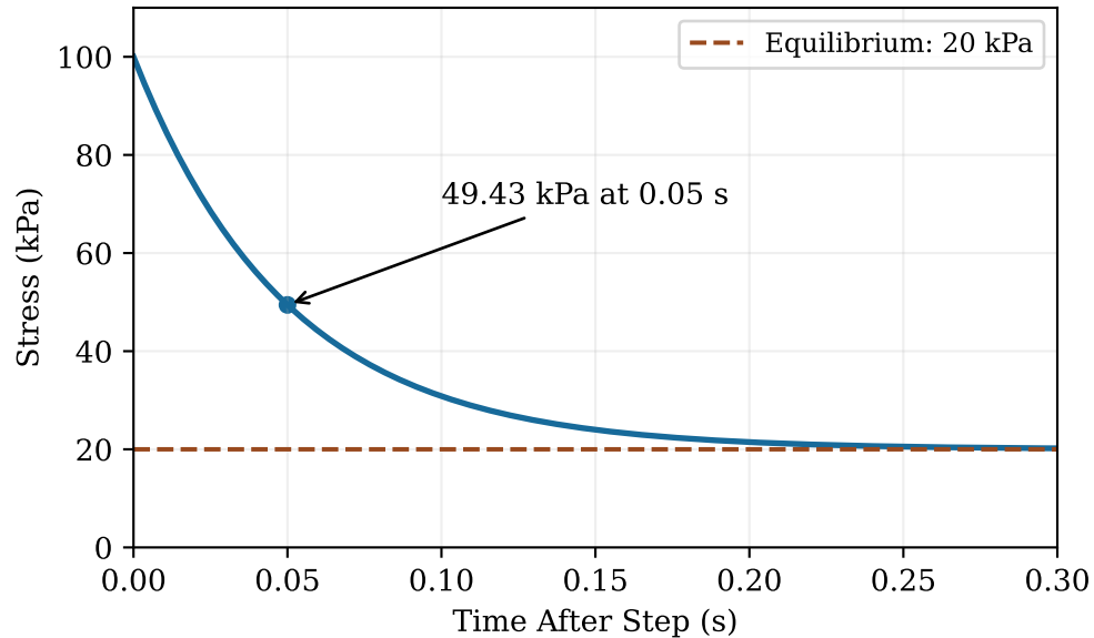
Held Strain: Stress Relaxes
