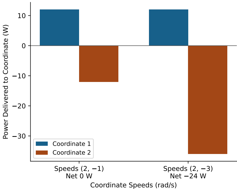
One Muscle, Two Power Outcomes
