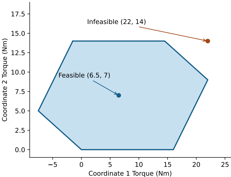
Coupled Torque Capacity
