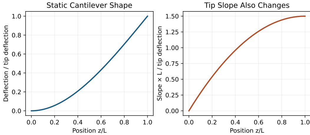
Figure 21.1: A Tip-Normalized Static Cantilever Shape and Its Slope. This Is an Admissible Approximation, Not an Exact Vibration Eigenmode.
