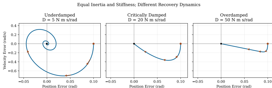
Figure 32.1: Manufactured Recovery With Equal Inertia and Stiffness: Only the Underdamped Case Spirals. All Curves Start at 0.1 rad With Zero Velocity; Orange Arrows Indicate Time Direction Over a Two-Second Interval.
