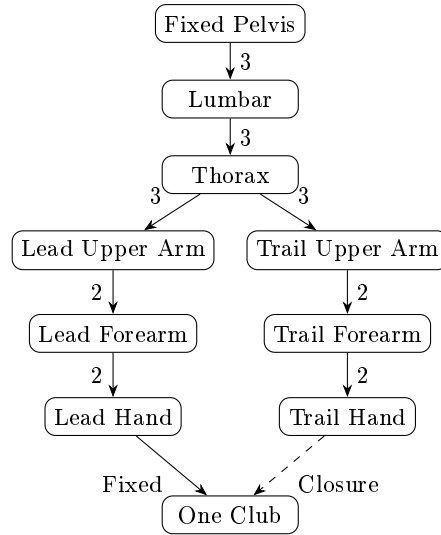
Figure 26.1: Upper-Body Tree and Two-Hand Closure. Numbers Indicate Compound-Joint Freedoms; the Dashed Connection Closes the Second Grip.
