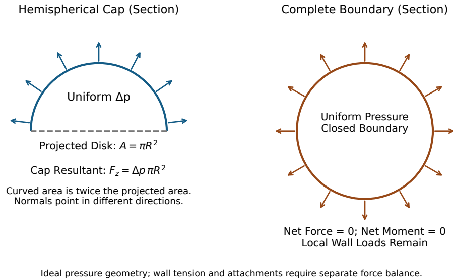
Figure 23.2: Pressure Acts Normal to a Surface. A Hemispherical Cap Has an Axial Resultant Based on Its Projected Disk; a Complete Uniform-Pressure Boundary Has Zero Net Force and Moment Despite Local Loading.
