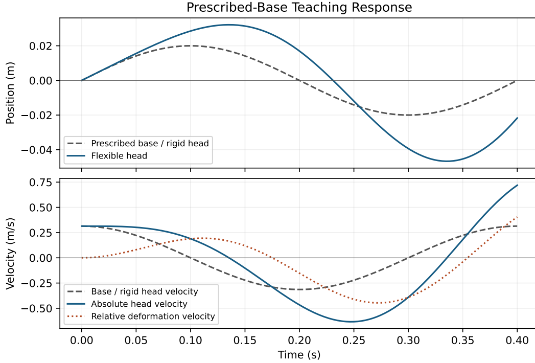
Figure 21.2: Position and Velocity Under the Declared Prescribed Base. The Flexible Response Includes Continuing Boundary Work; No Ball-Impact Event Is Modeled.
