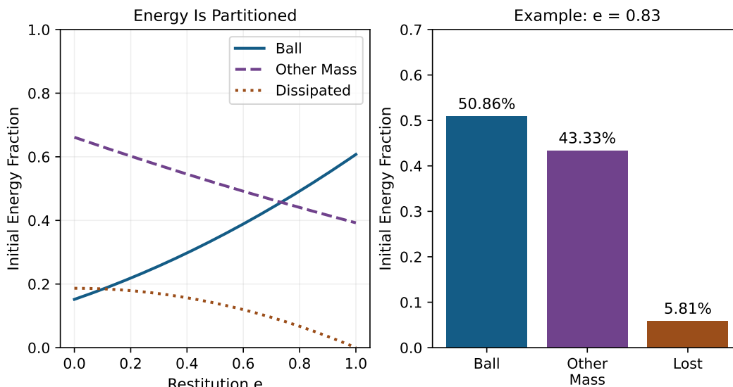
Figure 33.2: Restitution Does Not Equal Energy Transfer. The Free Two-Mass Teaching Model Uses a 0.200 kg Incoming Mass and a Stationary 0.04593 kg Ball; Fractions Sum to One.
