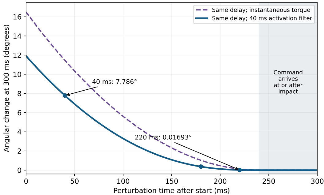
Figure 31.1: Remaining Time Changes the Same Command's Effect. The Declared Rotor Model Compares Instantaneous Torque With Activation Filtering After the Same 60ms Delay. These Are Illustrative Responses, Not Measured Golf Data.
