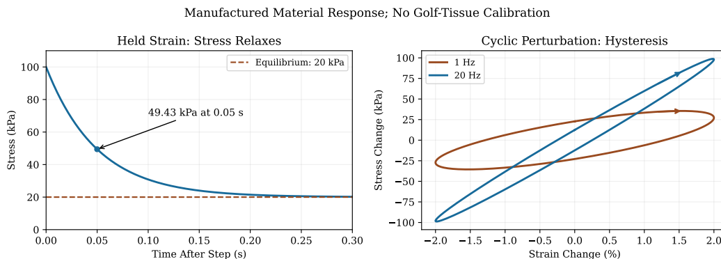
Figure 22.1: Manufactured Standard-Linear-Solid Response With Equilibrium Modulus 1 MPa, Branch Modulus 4 MPa and Relaxation Time 0.05 s. Left: An Ideal 2 Percent Strain Step. Right: Steady Cycles of 2 Percent Strain Amplitude About a Tensile Bias; Arrows Show Time Direction. These Curves Are Model Examples, Not Golf-Tissue Measurements.
