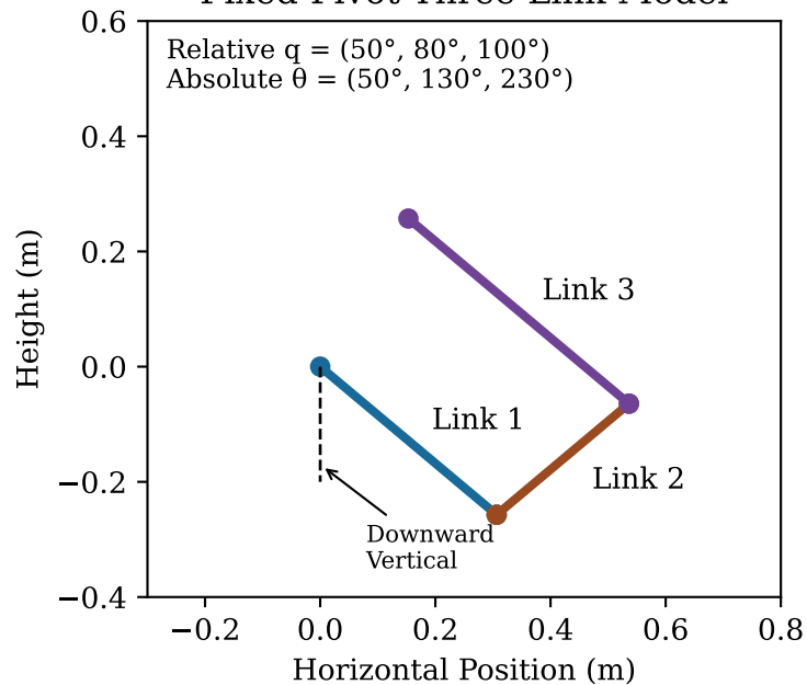
Fixed-Pivot Three-Link Model
