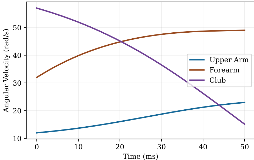
Zero-Torque Absolute Angular Rates
