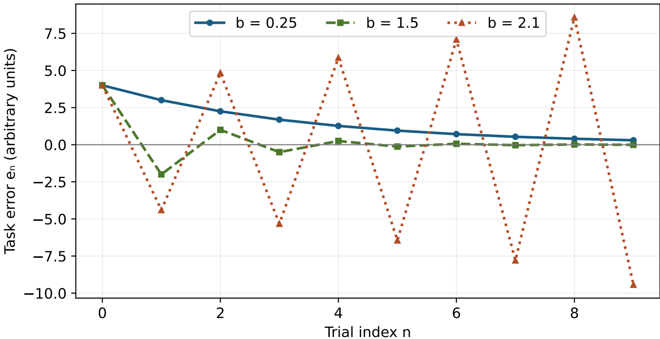
A Larger Update Can Destabilize Learning
