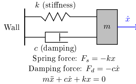
Figure 16.1: Parallel Spring and Damper Acting on a Translating Mass. Both Elements Share the Same Displacement and Velocity; Their Forces Add. An Angular Analogue Uses Rotational Inertia and Torques.
