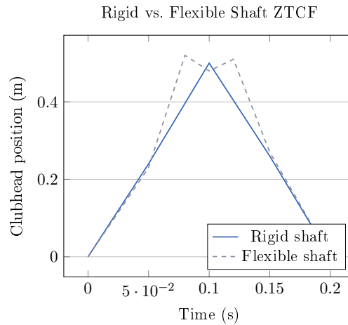
Figure 19.1: Qualitative comparison of rigid vs. flexible shaft ZTCF trajectories. The flexible shaft shows oscillation near the maximum height, characteristic of the catapult effect.
