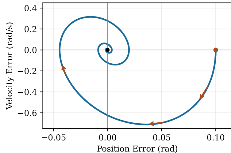
Underdamped D = 5 \text{ N m s/rad}
