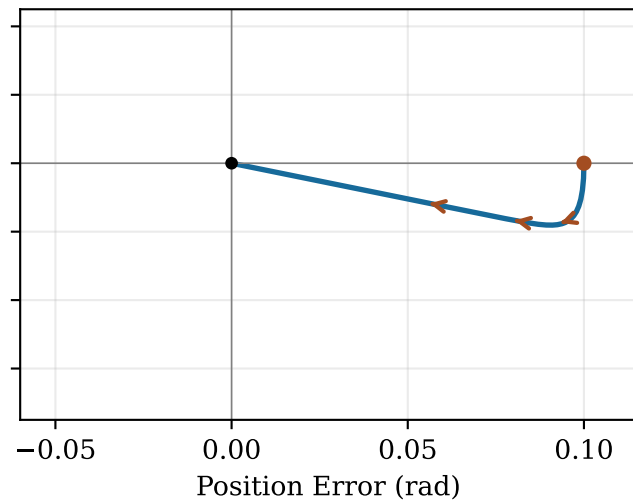
Overdamped D = 50 \text{ N m s/rad}
