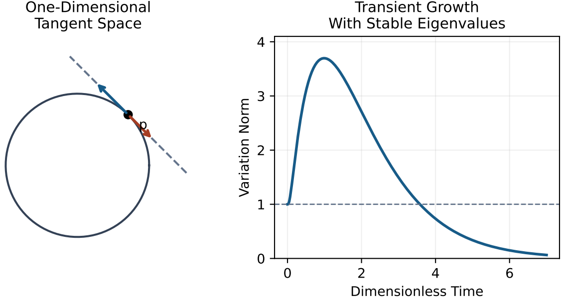
Figure 1.1: Tangent Vectors and Finite-Time Amplification. Left: A One-Dimensional Circle Has a Tangent Line. Right: A Stable Linear System Can Amplify a Variation Before It Decays.
