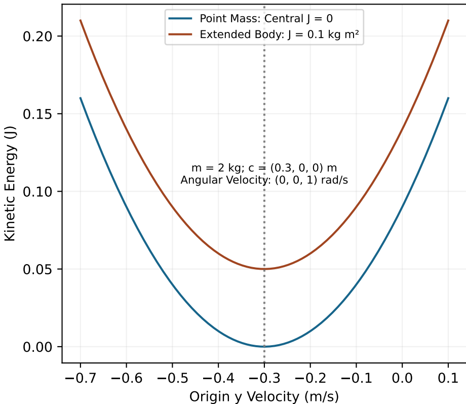
Energy Depends on the Mass Distribution
