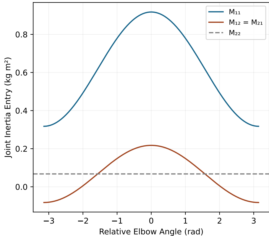
Articulation Changes the Joint Mass Matrix
