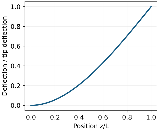
Static Cantilever Shape
