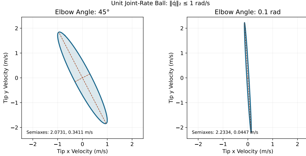
Figure 9.2: Position-Velocity Ellipses for Equal Unit-Length Links. Equal Plot Scales Reveal the Strong Anisotropy Already Present at 45 Degrees and Its Increase Near Extension.
