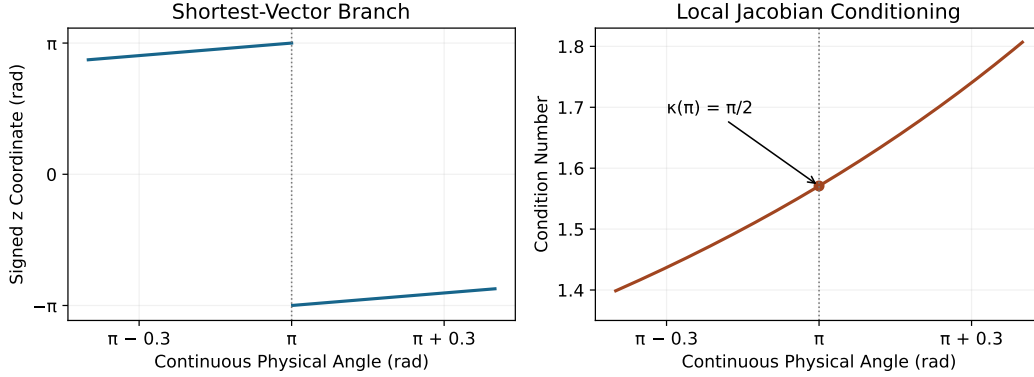
Figure 6.1: A Half-Turn Branch Cut Is Different From a Differential Singularity. A Smooth Rotation About a Fixed Axis Crosses the Shortest-Vector Cut, While the Chosen Local Jacobian Remains Nonsingular.
