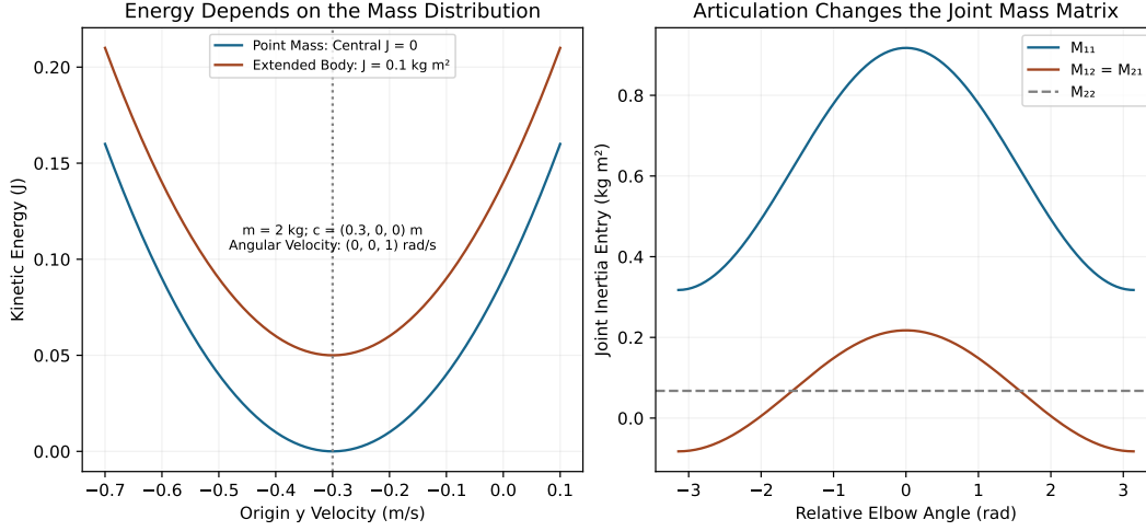
Figure 8.2: A Point Mass Has Zero-Energy Rotations About Itself; an Extended Body Also Has Rotational Energy. In the Two-Link Example, Elbow Configuration Changes the Joint Inertia and Its Coupling.
