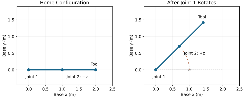
Figure 9.1: An Upstream Rotation Carries the Downstream Axis. The Home Axis Is a Constant Model Parameter; the Current Axis Passes Through the Moved Elbow.
