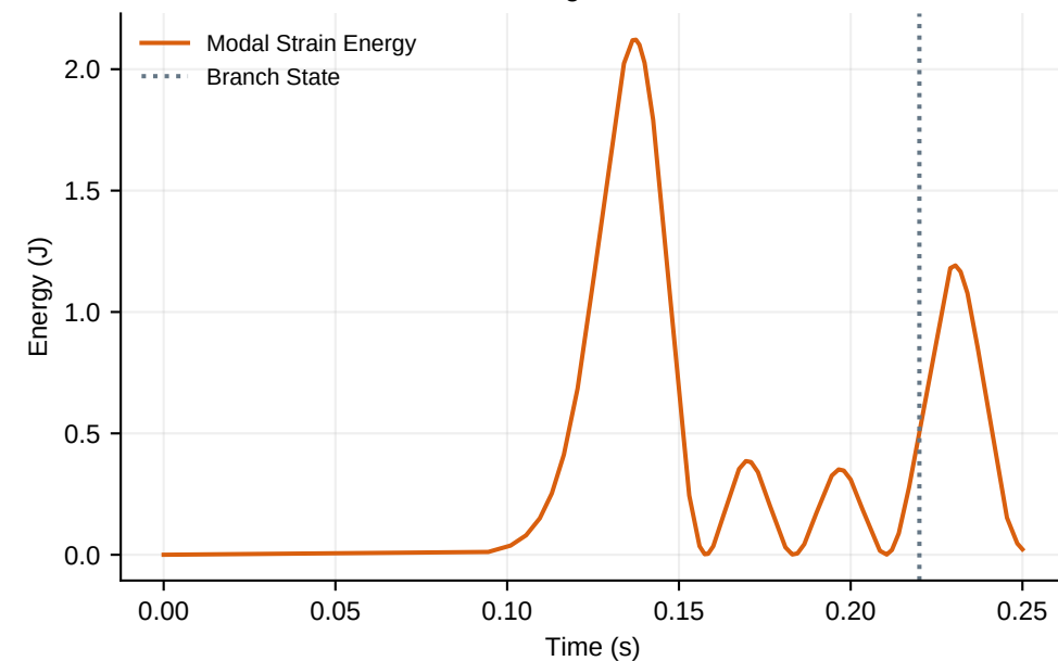
Baseline Modal Storage Before the Intervention
