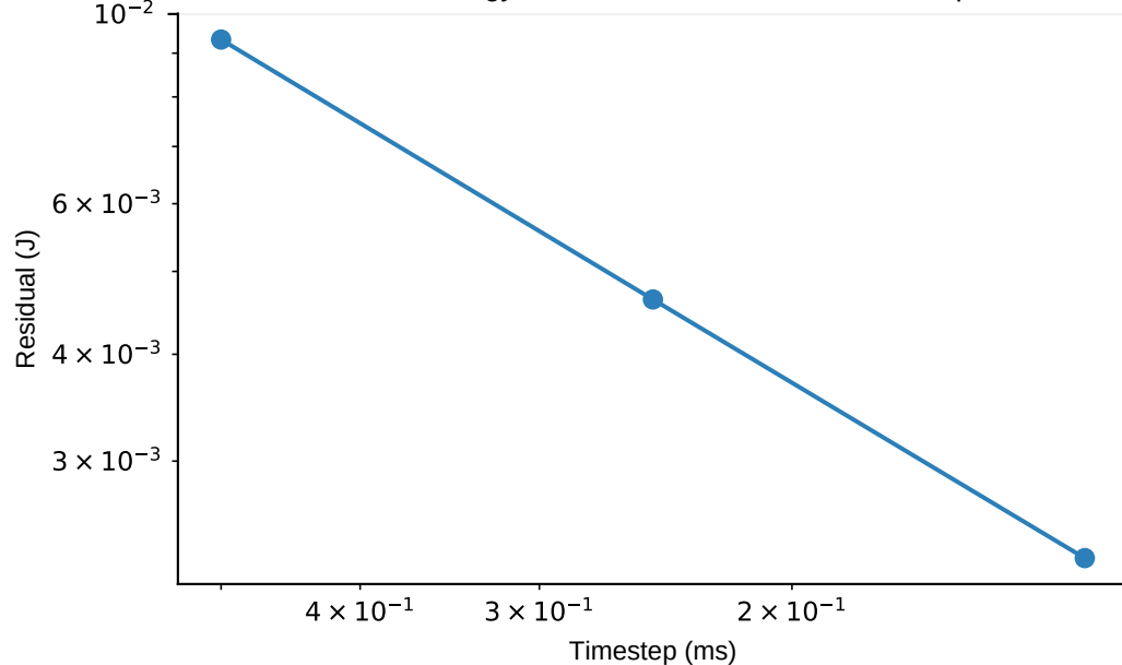
Work-Energy Residual Decreases with Timestep
