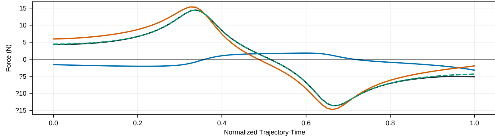
Two-Arm Net Mid-Grip Resultant
