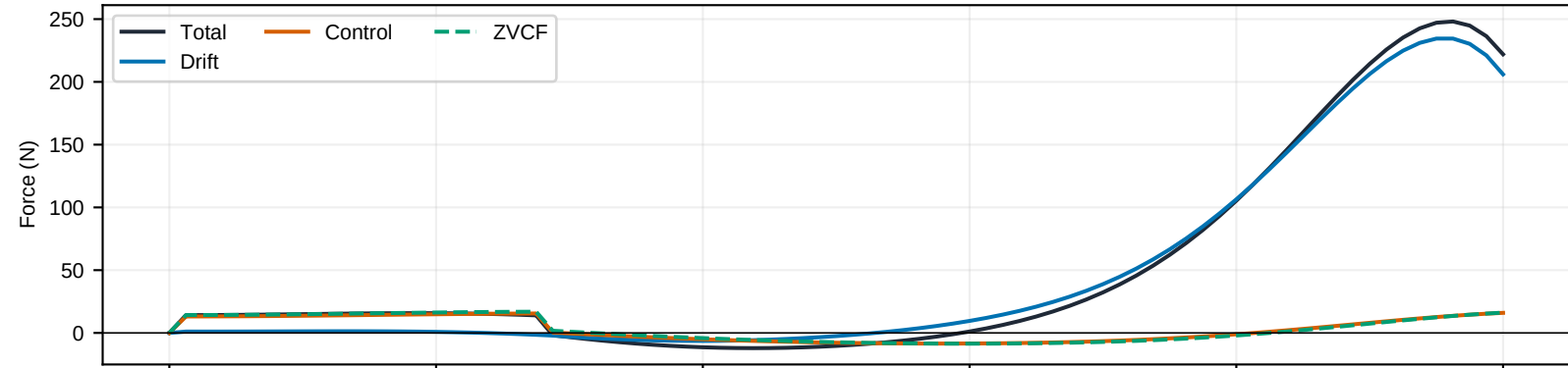
One-Arm Three-Link Net Club Force
