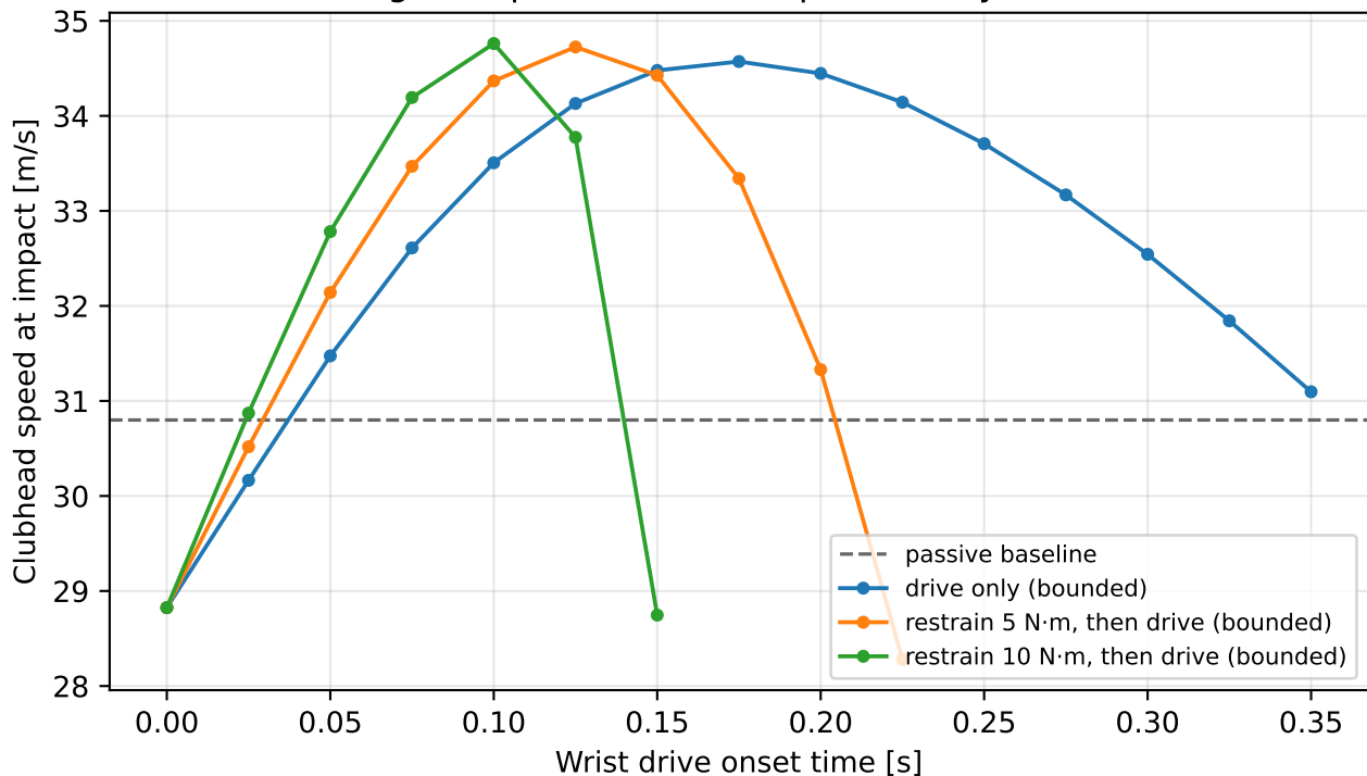
E1b — Timing sweep with linear torque-velocity bounds on drives
