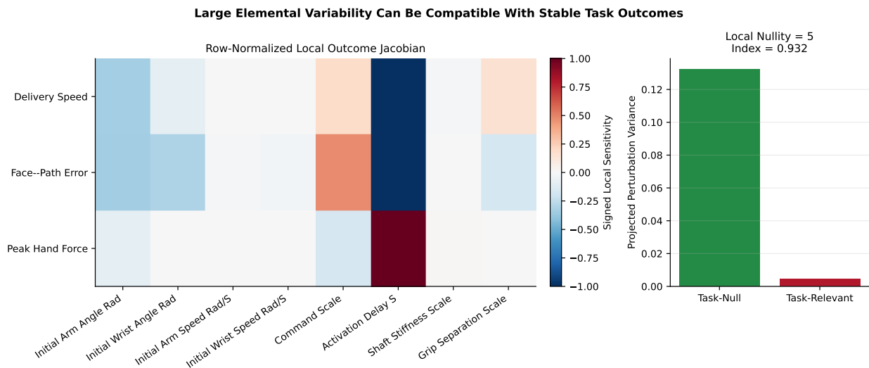
Figure 21.4: The local outcome Jacobian identifies task-sensitive input directions and a five-dimensional null space. This is a model input–outcome partition, not evidence of a neural synergy.
