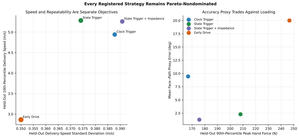
Figure 21.2: Held-out lower-tail speed and dispersion do not select the same program, and face/path error trades against peak hand force. Marker size in the left panel increases with peak-force exposure.
