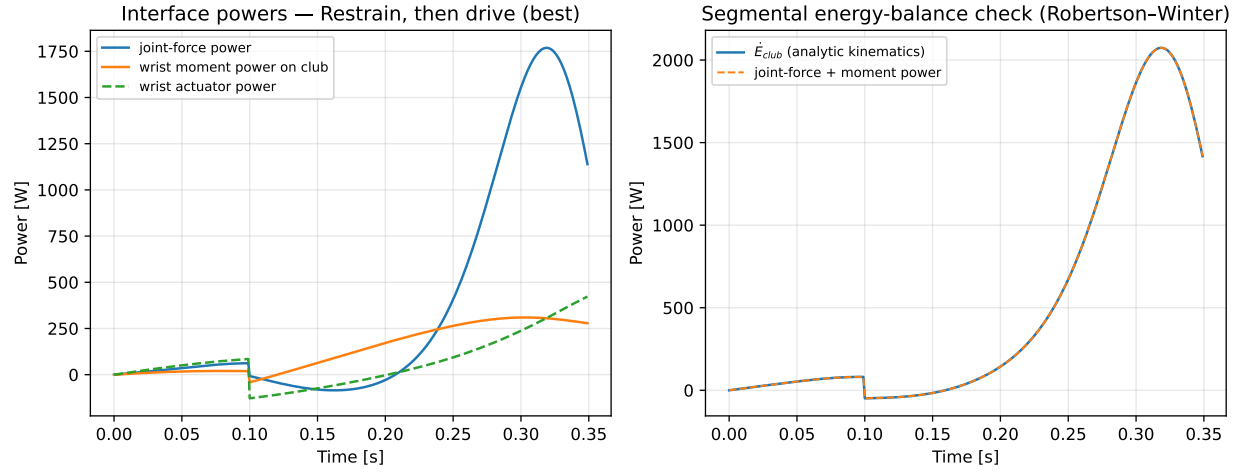
Figure 24.7: Left: wrist-interface powers for the best restrain-then-drive swing. Right: segmental energy-balance check — club mechanical-energy rate versus the sum of interface powers. The right-panel equality is pointwise after replacing sampled-velocity differentiation with analytic COM acceleration.
