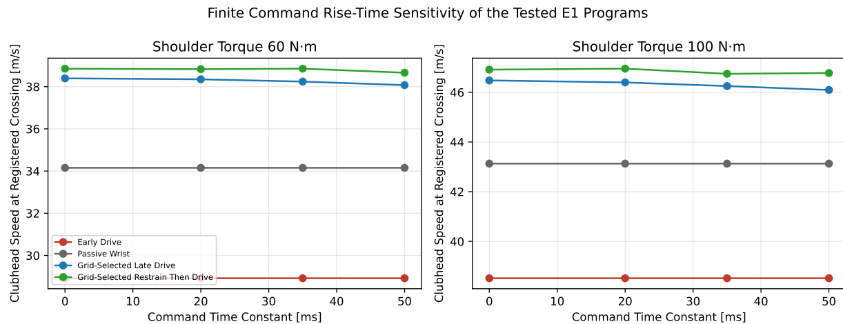
Figure 24.9: Finite Command Rise-Time Sensitivity of the Tested E1 Programs
