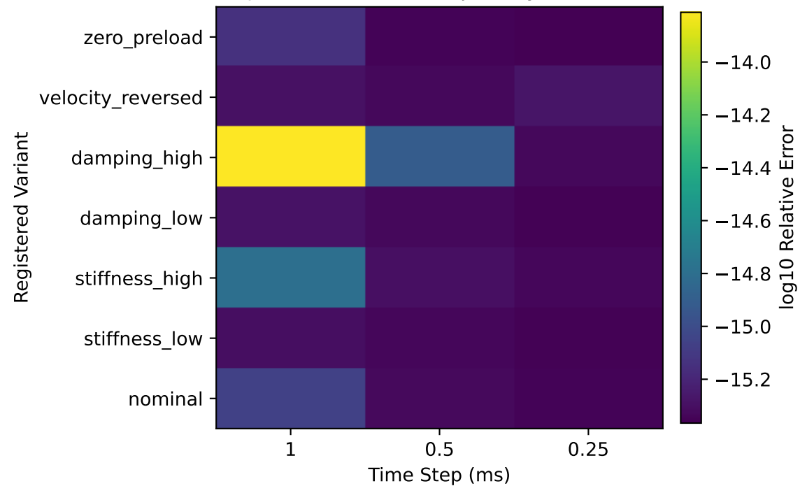
MuJoCo--Pinocchio Trajectory Difference
