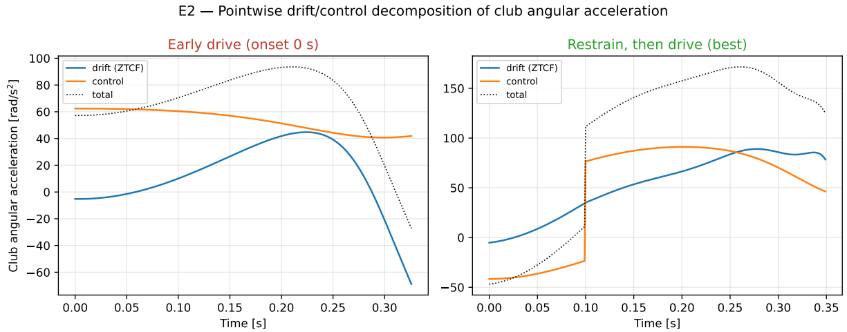
Figure 25.8: Pointwise drift (ZTCF) versus control decomposition of club absolute angular acceleration, for the early-drive (left) and best restrain-then-drive (right) programs.
