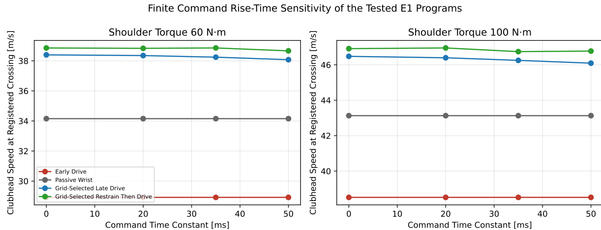
Figure 25.9: Finite Command Rise-Time Sensitivity of the Tested E1 Programs
