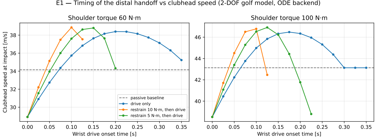
Figure 25.1: E1 sweep: clubhead speed at impact versus wrist-drive onset time, for drive-only and restrain-then-drive profiles at two shoulder-torque levels. Dashed line: fully passive wrist baseline.
