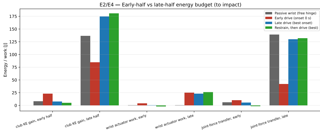
Figure 25.6: Early-half versus late-half energy budget (club kinetic-energy gain, wrist actuator work, integrated joint-force transfer) for the representative programs.
