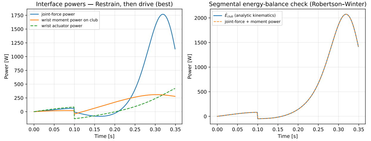
Figure 25.7: Left: wrist-interface powers for the best restrain-then-drive swing. Right: segmental energy-balance check — club mechanical-energy rate versus the sum of interface powers. The right-panel equality is pointwise after replacing sampled-velocity differentiation with analytic COM acceleration.
