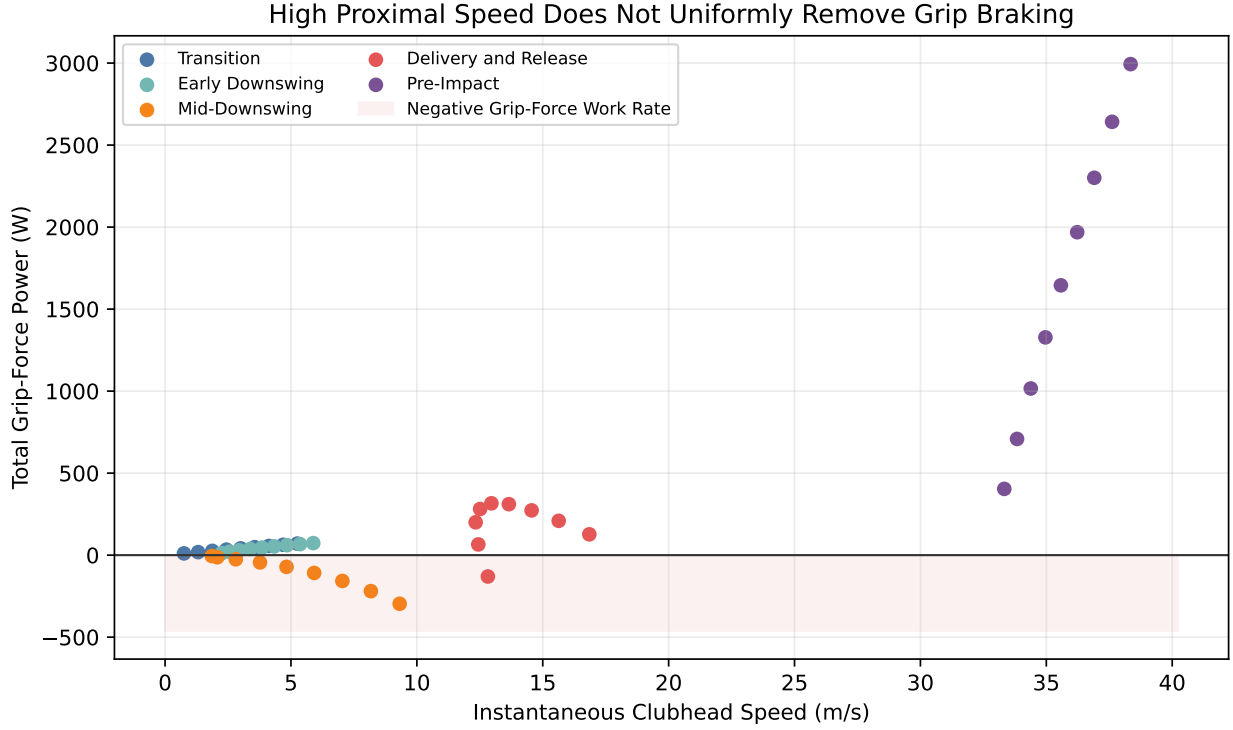
Figure 6.2: Negative grip power across phase and velocity-matching rule. Shading marks states in which the grip reaction removes modeled mechanical energy from the club at that instant.
