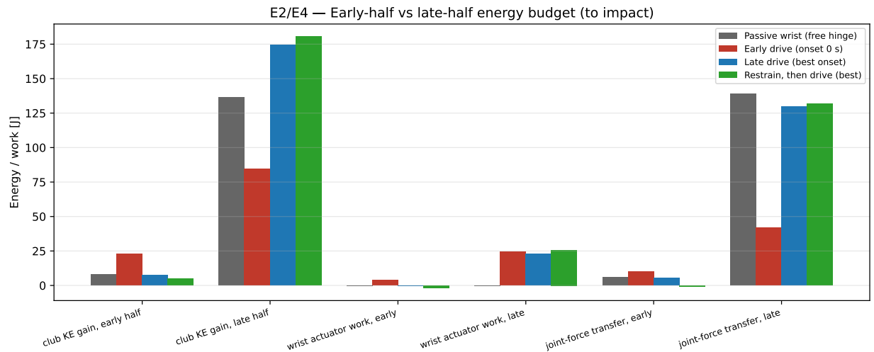
Figure 10.6: Early-half versus late-half energy budget (club kinetic-energy gain, wrist actuator work, integrated joint-force transfer) for the representative programs.
