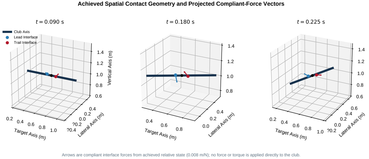
Figure 17.1: Achieved Spatial Contact Geometry and Projected Compliant-Force Vectors
