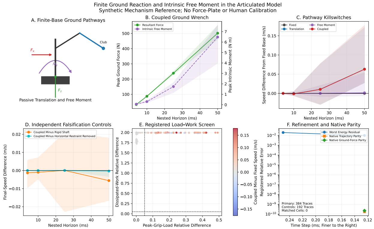
Figure 16.15: Finite Ground Reaction and Intrinsic Free Moment in the Articulated Model
