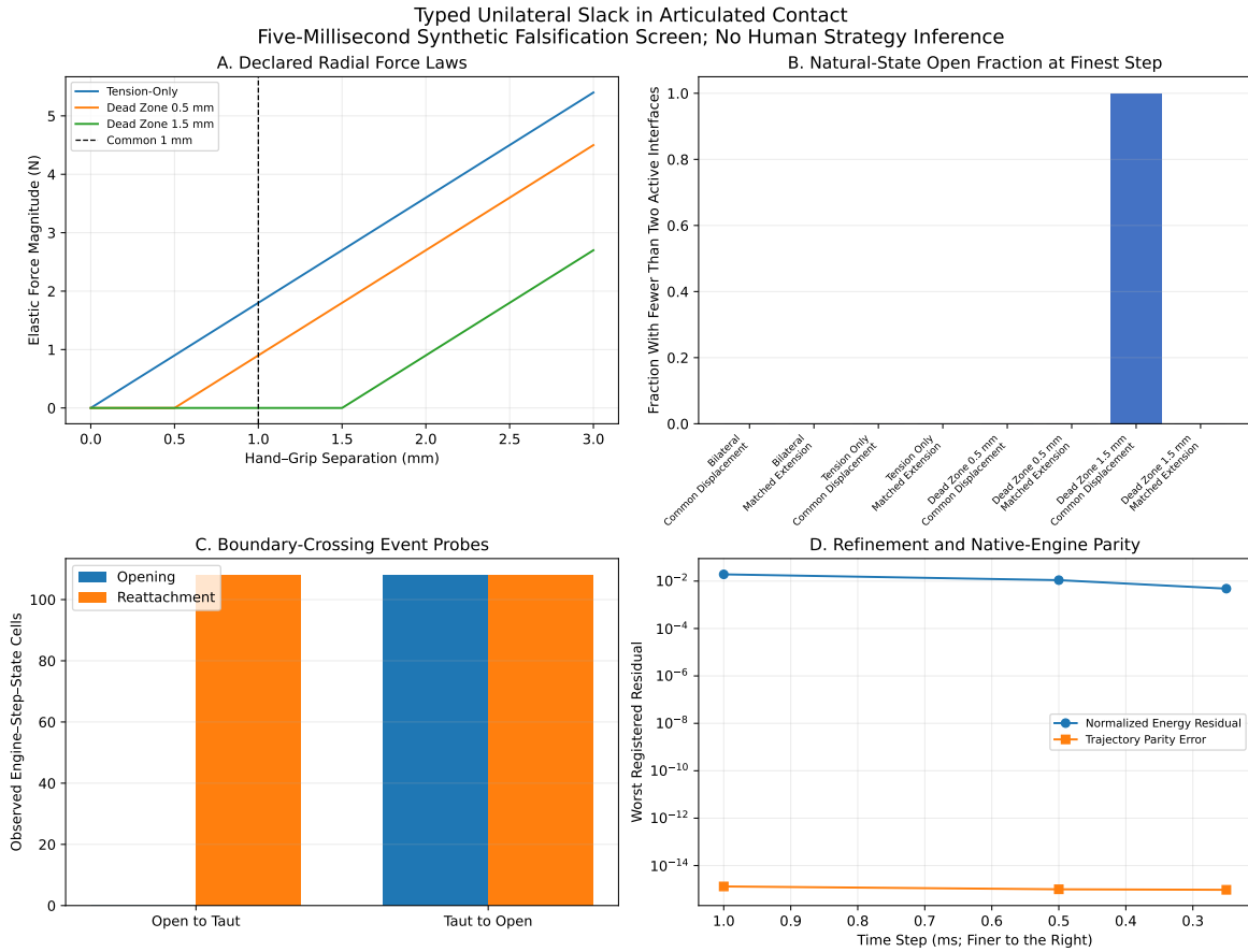
Figure 16.12: Typed Unilateral Slack and Reattachment Across Natural-State and Boundary-Crossing Controls
