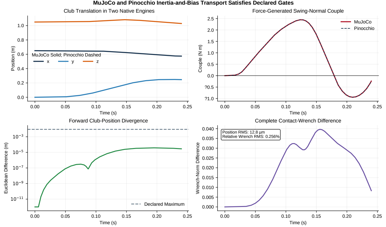
Figure 17.2: MuJoCo and Pinocchio Inertia-and-Bias Transport Satisfies Declared Gates
