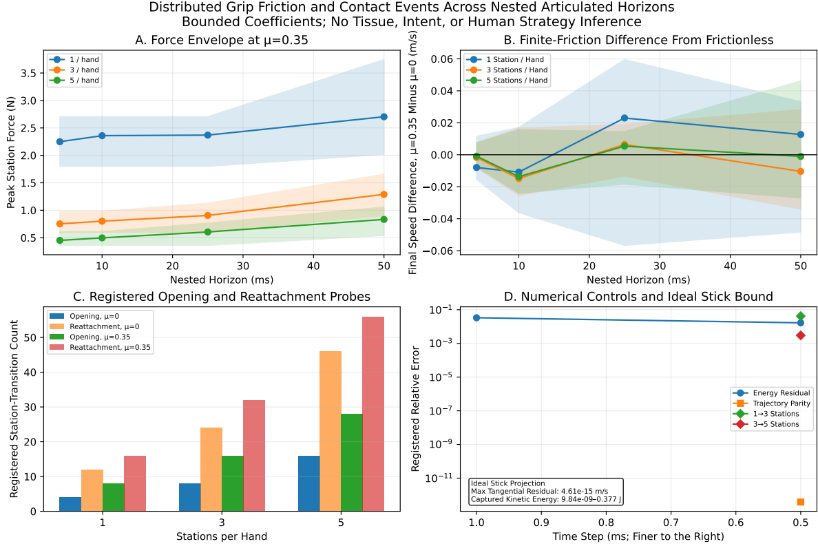
Figure 16.13: Distributed Grip Friction and Contact Events Across Nested Articulated Horizons
