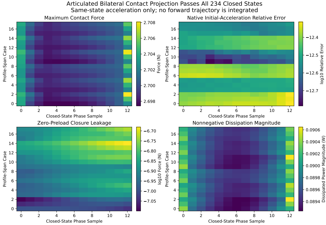
Figure 16.10: Articulated Contact Projection and Initial Acceleration Across All Closed States
